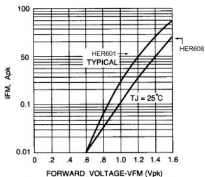
Fig. 2 - FORWARD CHARACTERISTICS
