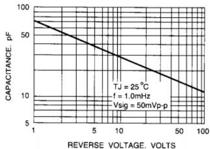
FIG. 5 - TYPICAL JUNCTION CHARACTERISTICS
