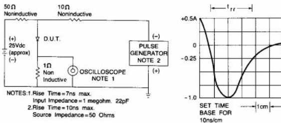
FIG. 5 - REVERSE RECOVERY TIME CHARACTERISTIC AND TEST DIAGRAM
