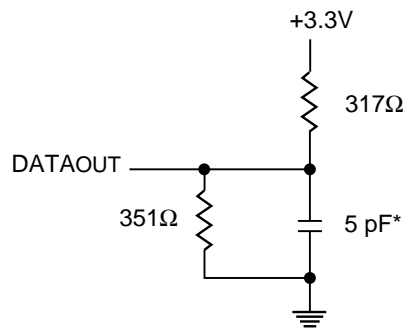
Figure 2. Output Load
