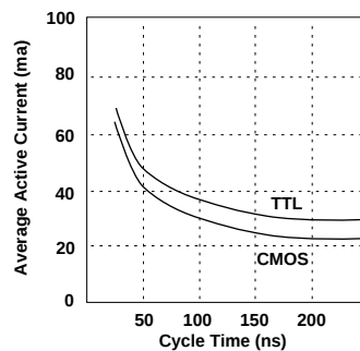
Figure 3 \text{I}_{\text{CC}} (Max) Writes
