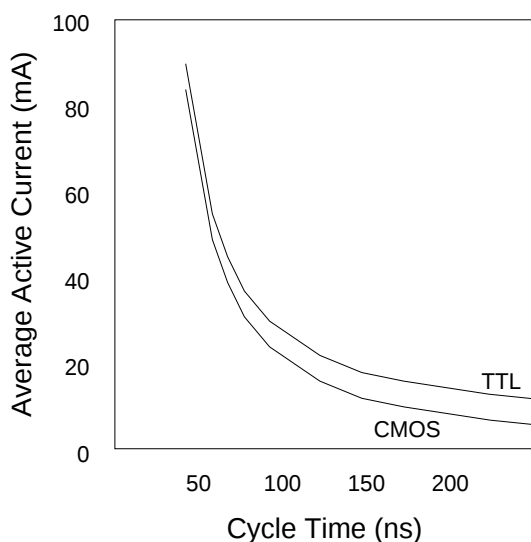
Fig 2: Icc (max) Reads
