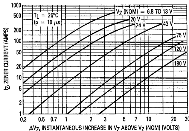
Figure 3. Dynamic Impedance
