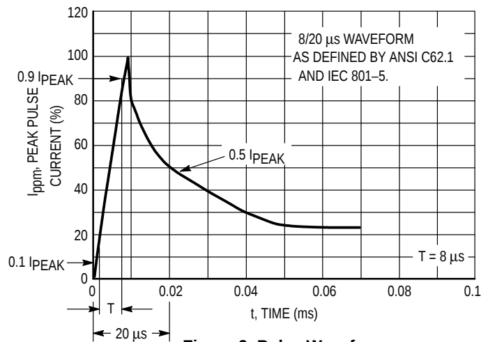
Figure 9. Pulse Waveform
