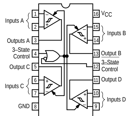
PIN CONNECTIONS
