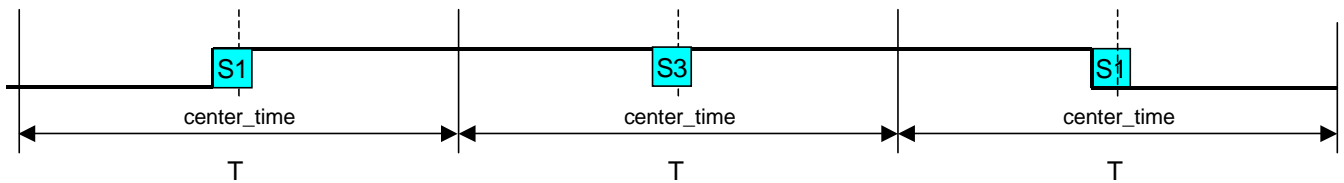
Figure 11. svmStdDtXor_res timing
