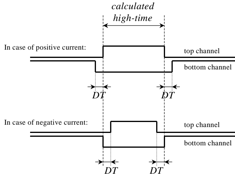
Figure 2. Dead-Time Correction Technique
