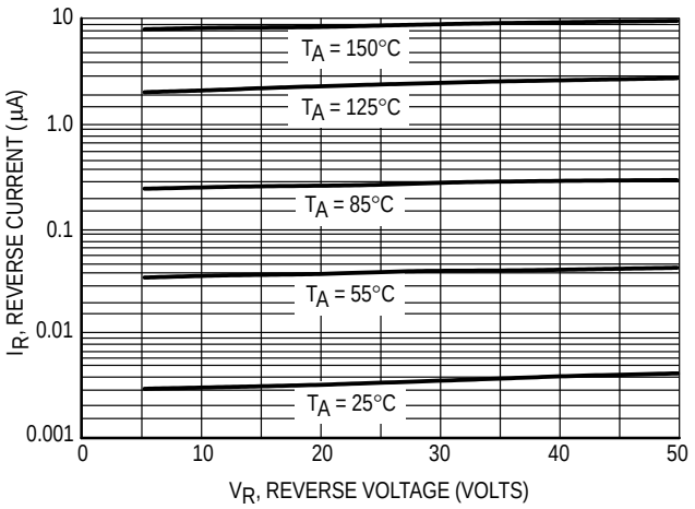
Figure 2. Leakage Current
