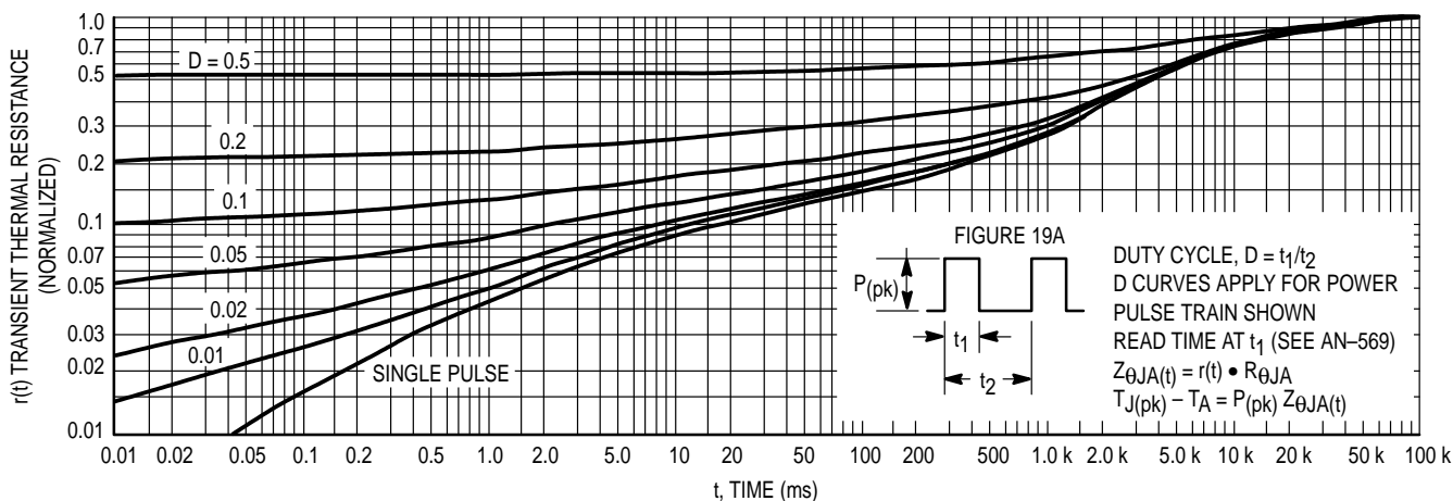
Figure 16. Thermal Response
