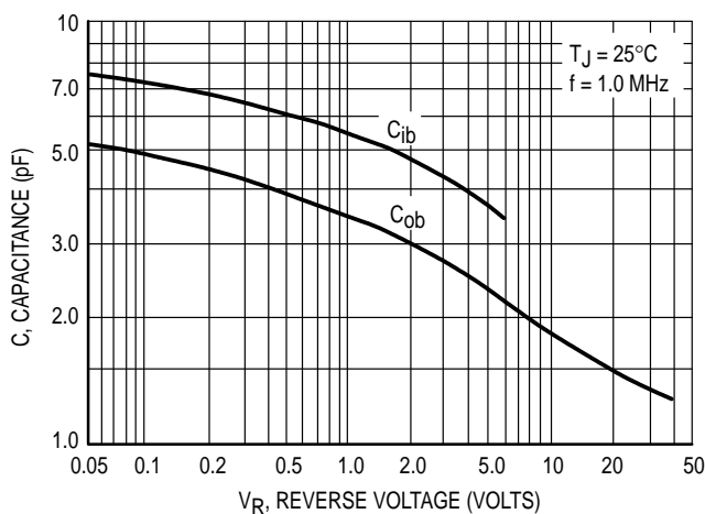
Figure 15. Capacitance
