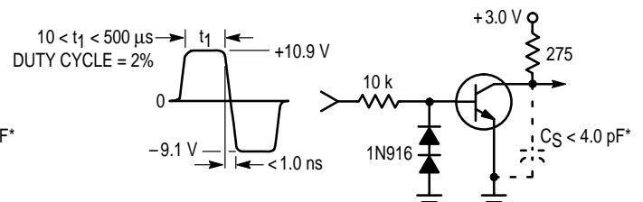
Figure 2. Turn–Off Time
