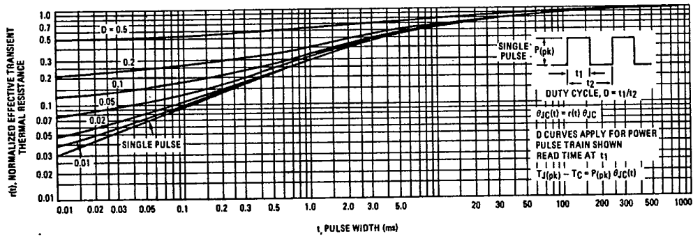
FIGURE 5 — THERMAL RESPONSE
