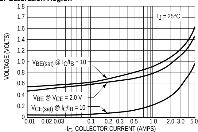
Figure 4. "On" Voltage
