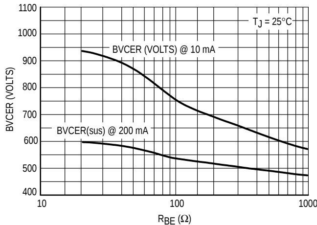
Figure 23. BVCEr
