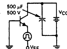
FIGURE 18 - OVERLOAD SOA TEST CIRCUIT
