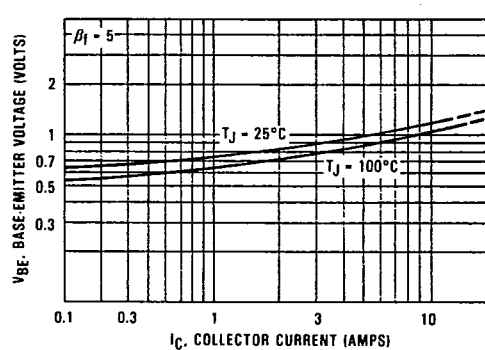
FIGURE 4 - BASE-EMITTER VOLTAGE
