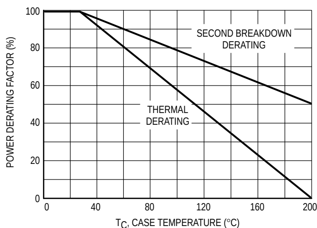
Figure 14. Power Derating
