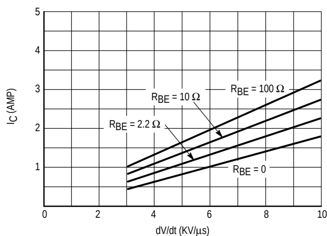
Figure 17. I_C = f(dV/dt)
