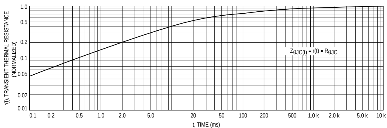
FIGURE 8 – THERMAL RESPONSE
