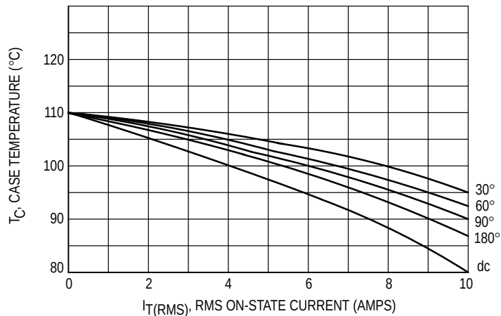
Figure 1. RMS Current Derating
