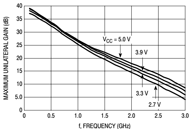
Figure 5. GUmux versus Frequency
