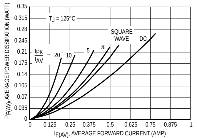
Figure 6. Power Dissipation
