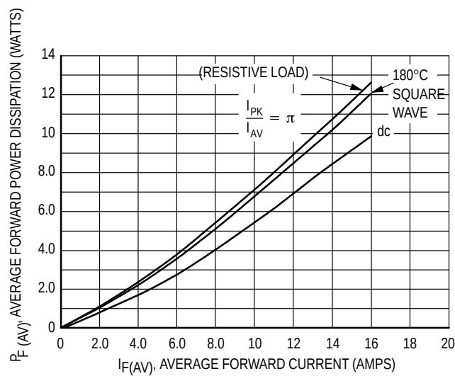
Figure 5. Power Dissipation
