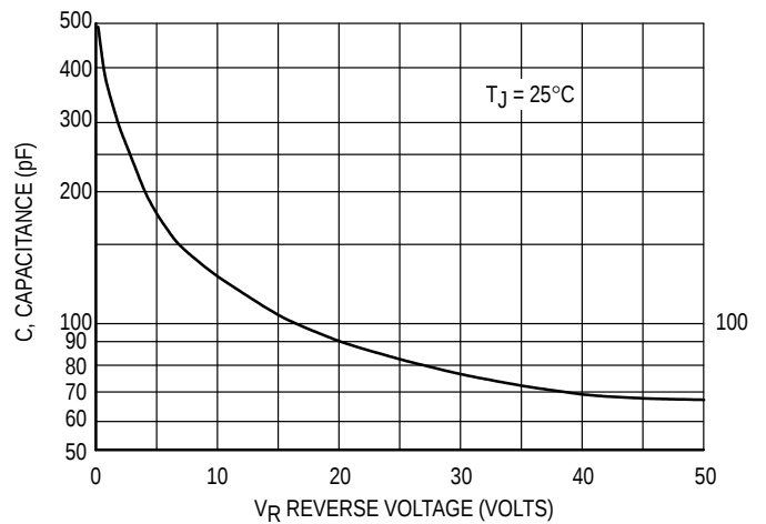
Figure 5. Typical Capacitance
