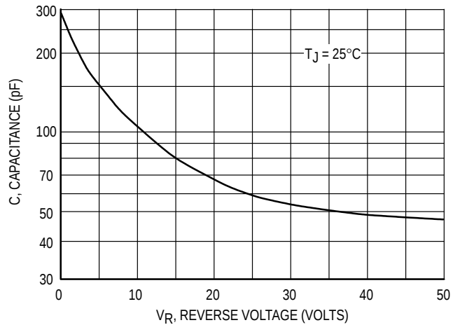
Figure 10. Typical Capacitance
