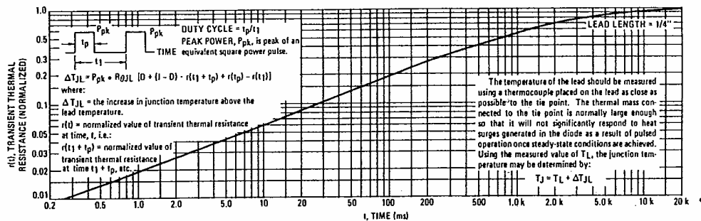
FIGURE 5 -- THERMAL RESPONSE
