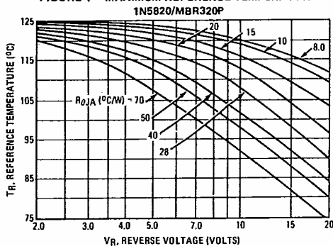
FIGURE 3 – MAXIMUM REFERENCE TEMPERATURE
