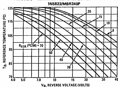
FIGURE 3 – MAXIMUM REFERENCE TEMPERATURE
