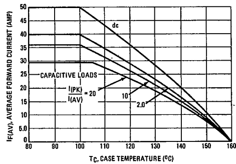
FIGURE 7 - CURRENT DERATING
