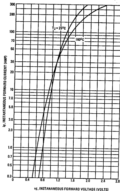
FIGURE 1 — FORWARD VOLTAGE
