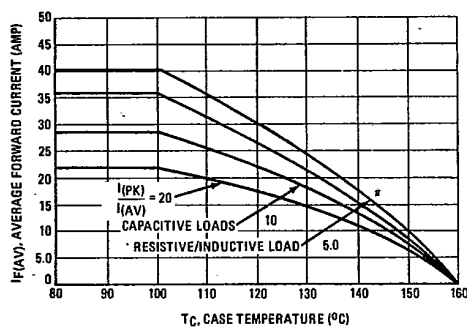
FIGURE 6 - CURRENT DERATING
