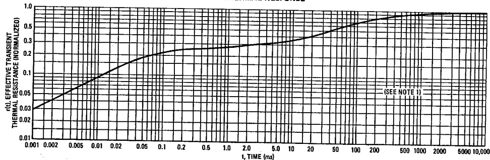
FIGURE 3 — THERMAL RESPONSE
