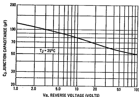
FIGURE 11 — JUNCTION CAPACITANCE
