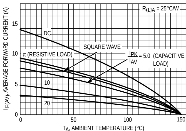
Figure 7. Current Derating
