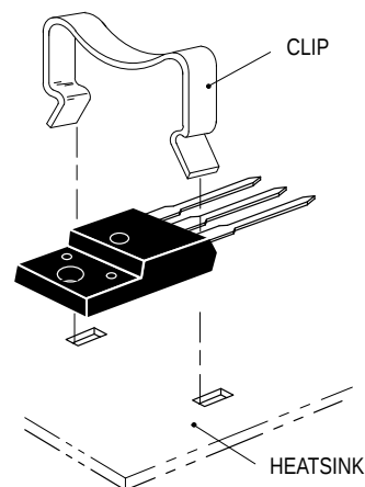
Figure 6b. Clip-Mounted
