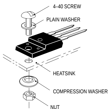
Figure 6a. Screw-Mounted
