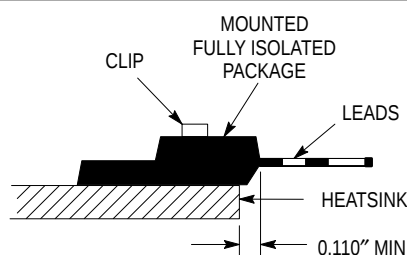
Figure 3. Screw or Clip Mounting Position for Isolation Test Number 1
