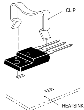
8b. Clip-Mounted
