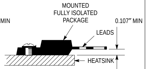
Figure 7. Screw Mounting Position for Isolation Test Number 3
