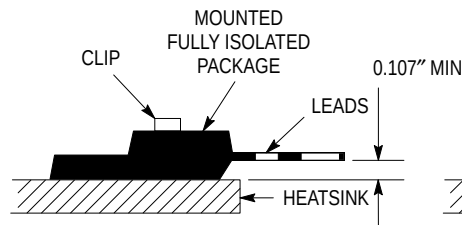
Figure 6. Clip Mounting Position for Isolation Test Number 2
