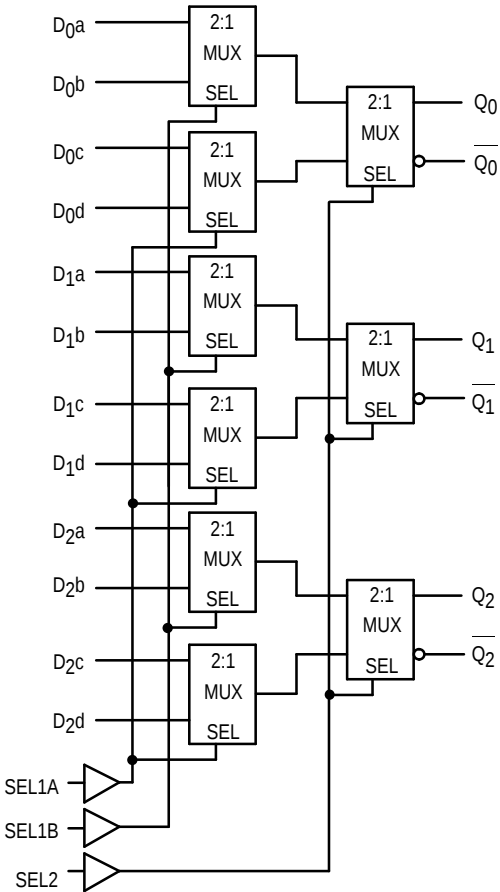
LOGIC DIAGRAM
