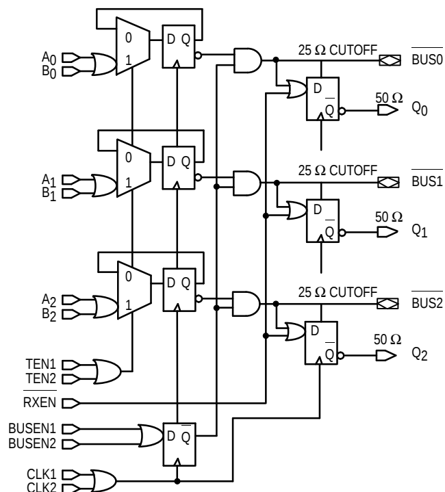
LOGIC DIAGRAM
