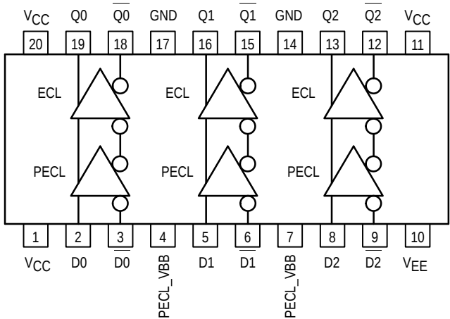
Figure 1. 20-Lead Pinout (Top View) and Logic Diagram
