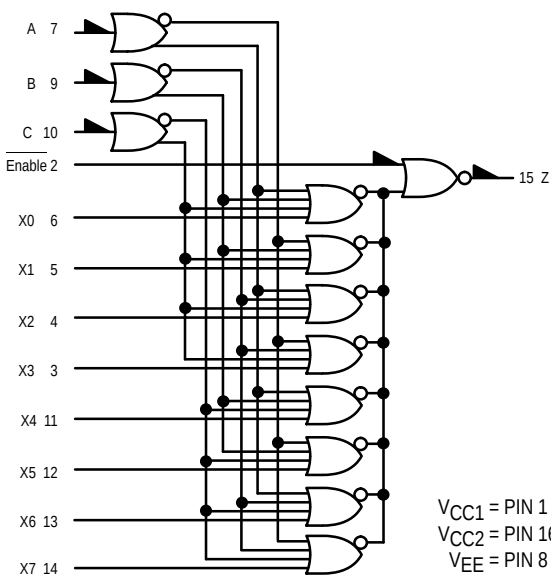
LOGIC DIAGRAM
