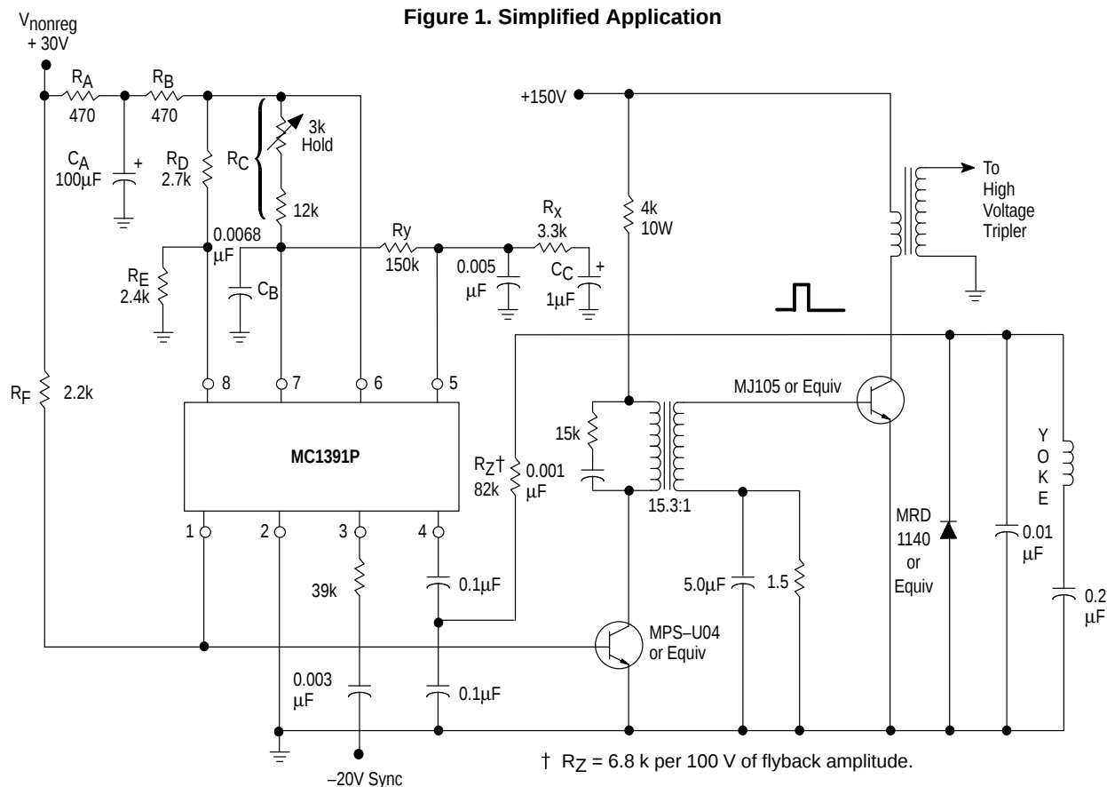
Figure 1. Simplified Application
