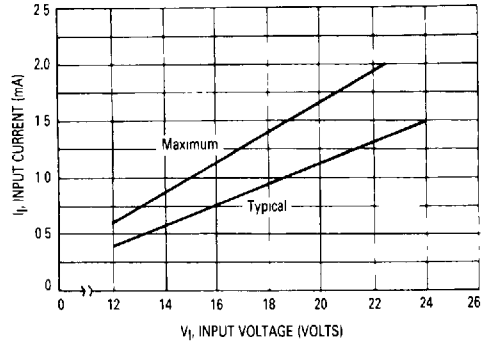
FIGURE 6 — INPUT CHARACTERISTICS — MC1416,B
