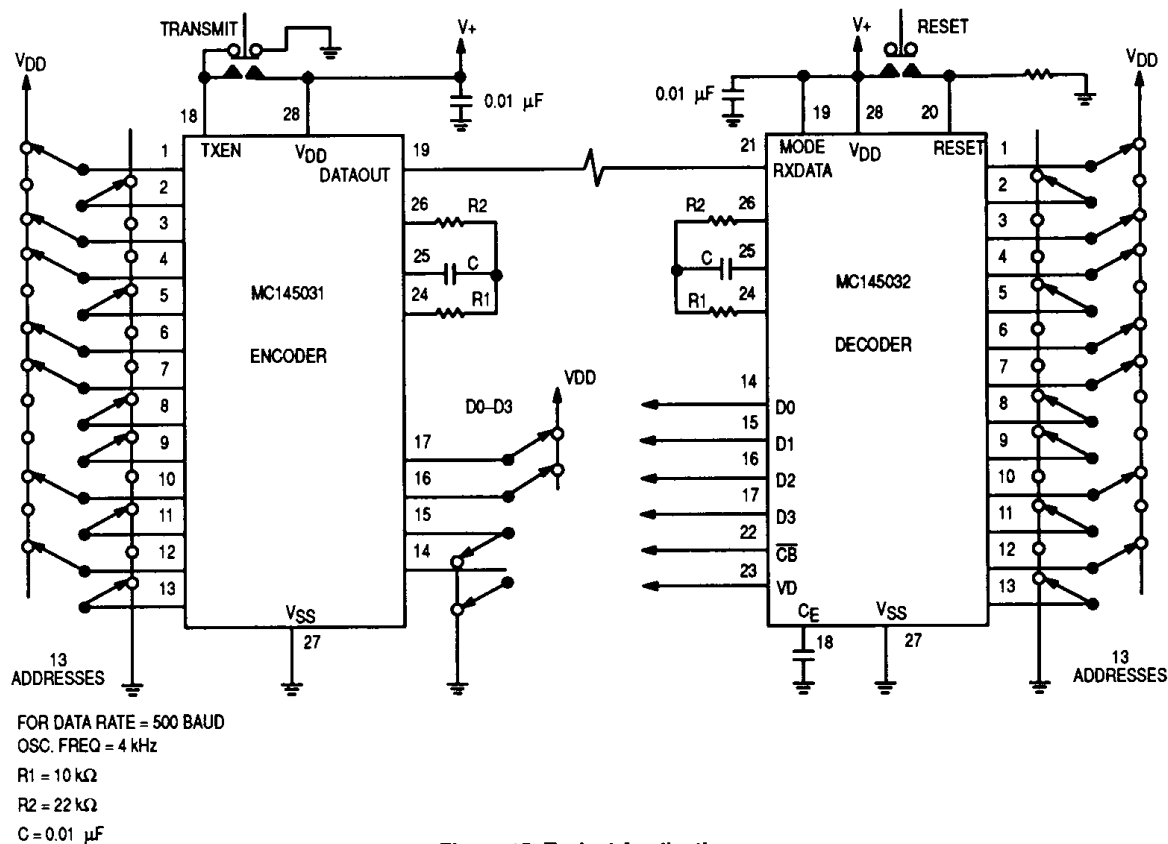
Figure 15. Typical Application
