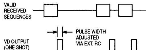
Figure 5. Valid Address Output Timing (MC145035)
