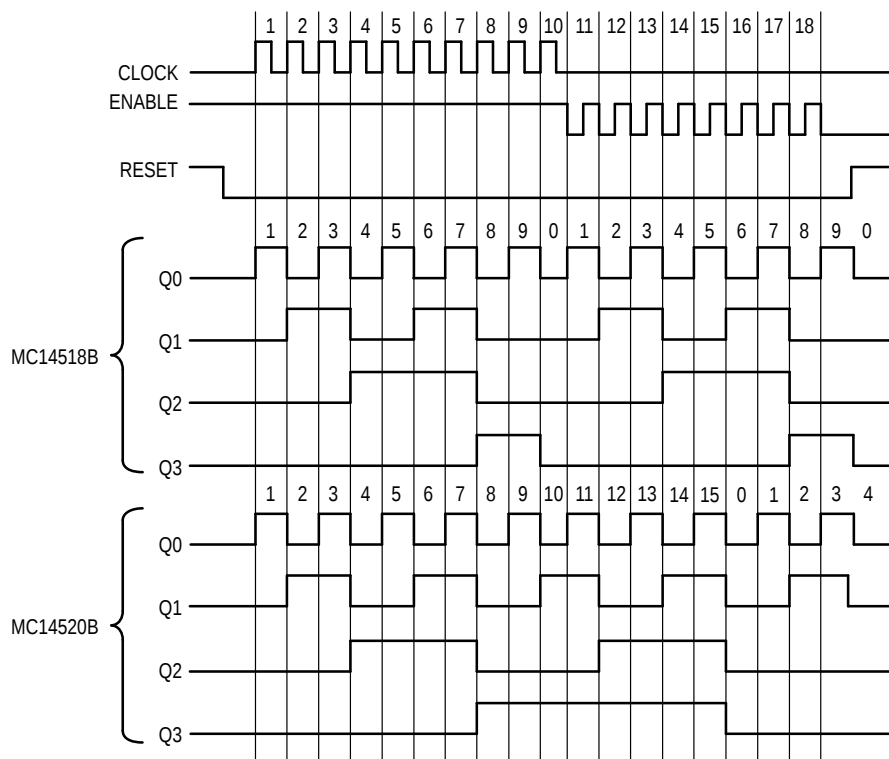
Figure 3. Timing Diagram
