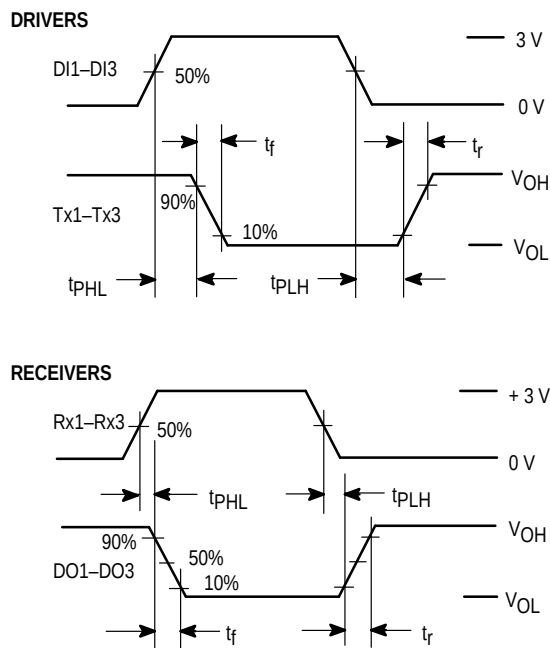
Figure 2. Switching Characteristics
