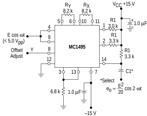
Figure 28. Frequency Doubler
