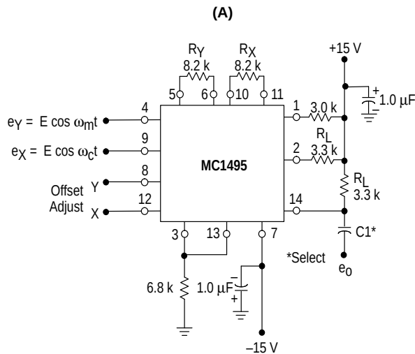
Figure 29. Balanced Modulator
