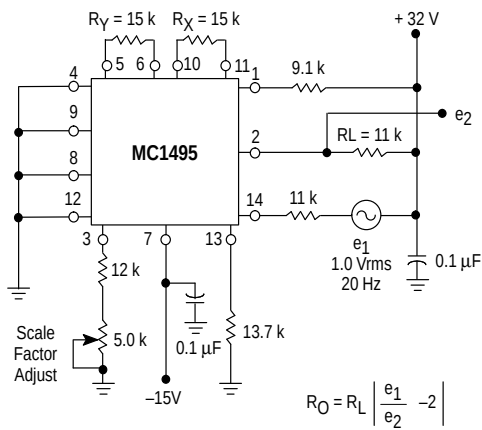
Figure 8. Output Resistance
