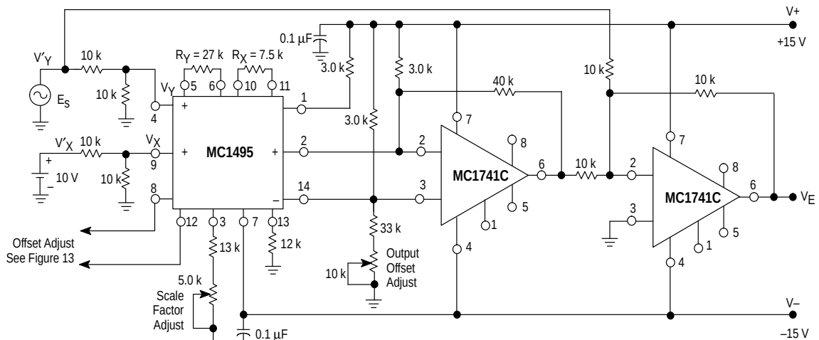
Figure 4. Linearity (Using Null Technique)
