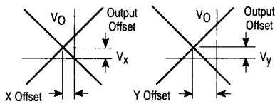
X, Y and Output Offset Voltages
