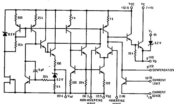
FIGURE 1 - CIRCUIT SCHEMATIC
