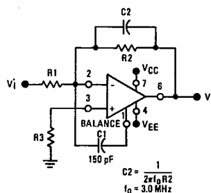
FIGURE 4 - FEEDFORWARD COMPENSATION
