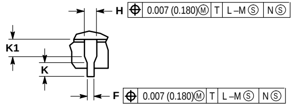
VIEW S
