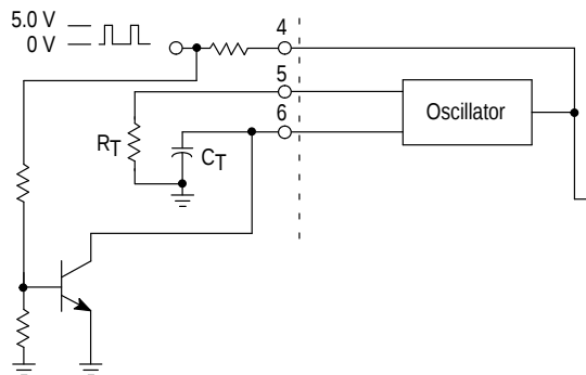
Figure 24. External Clock Synchronization
