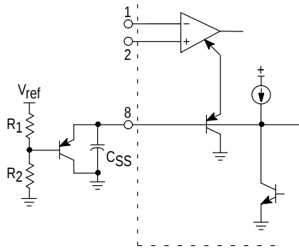
Figure 31. Buffered Maximum Clamp Level
