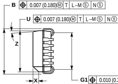
VIEW D-D
