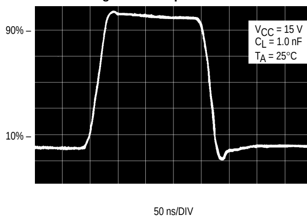
Figure 12. Output Waveform
