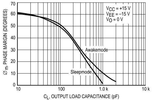
Figure 26. Phase Margin versus Output Load Capacitance
