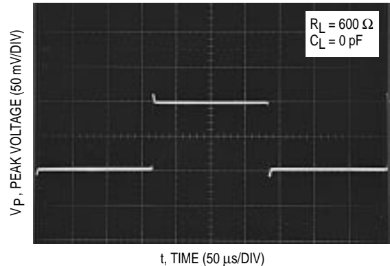
Figure 38. Awakemode Small Signal Transient Response
