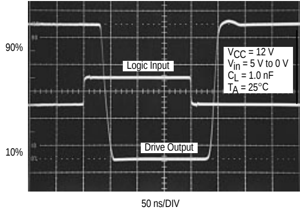
Figure 7. Propagation Delay
