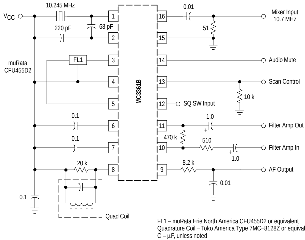
Figure 1. Test Circuit
