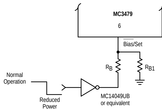
Figure 12. Power Reduction
