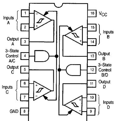
PIN CONNECTIONS
