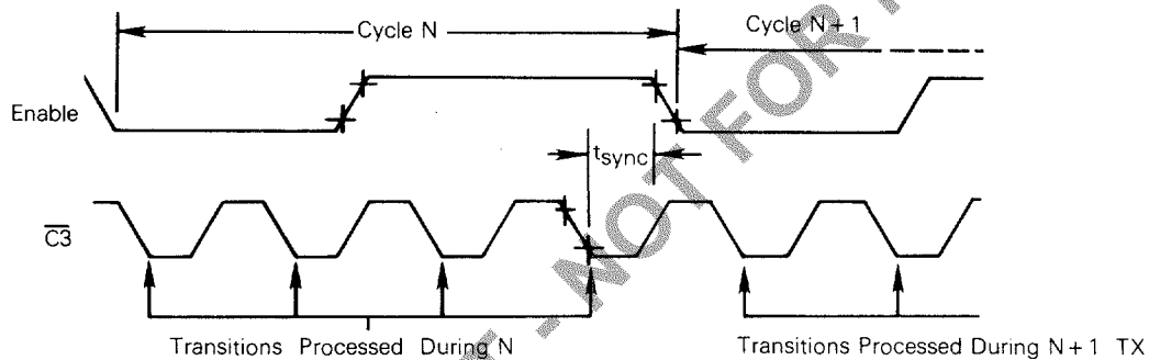
FIGURE 7 — \overline{C3} INPUT SYNCHRONIZATION TIME ( \div 8 PRESCALER MODE ONLY)
